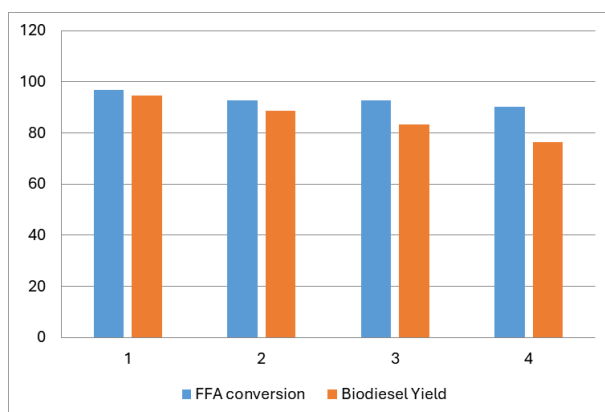
Figure 11. Impact of catalyst reusability on the biodiesel yield and FFA conversion of JSO
